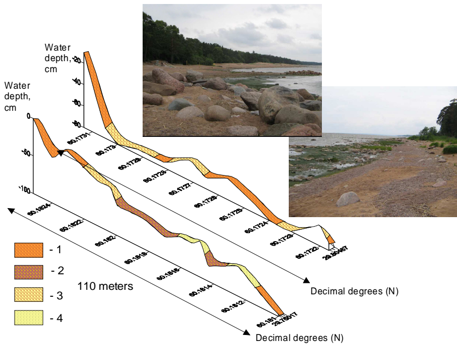
Fig.3. Near-shore profile of erosion zone. 1 – boulders, pebbles, gravel; 2 – sands with boulders; 3 – glacial till; 4 – fine-grained sand.
