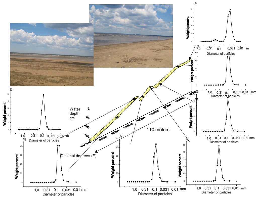
Fig.5. Near-shore profile of erosion zone. 1 – boulders, pebbles, gravel; 2 – sands with boulders; 3 - fine-grained sand.
