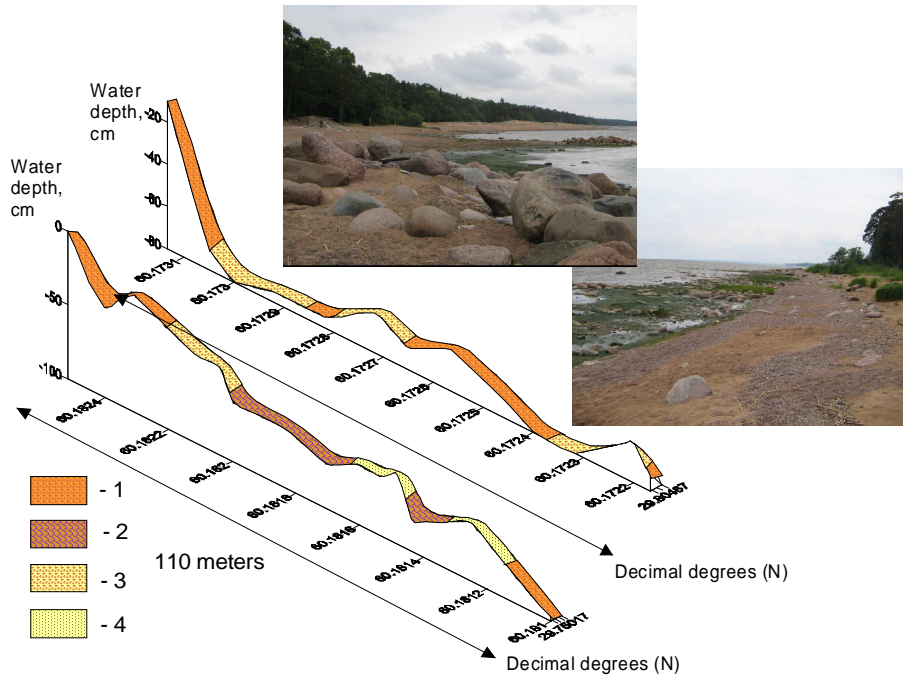
Fig.4. Near-shore profile of erosion zone. 1 – boulders, pebbles, gravel; 2 – sands with boulders; 3 – glacial till; 4 – fine-grained sand.
