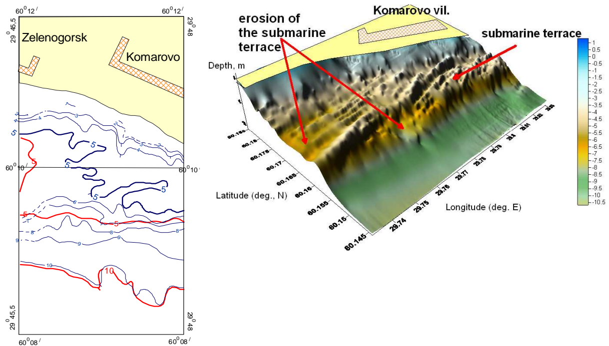
Fig. 10. Alteration of the depths in the near-shore zone as a result of the submarine terrace erosion. Red lines – isobaths of the navigational chart edited in 1989, blue lines – results of the depth measurements made by VSEGEI in 2005.
