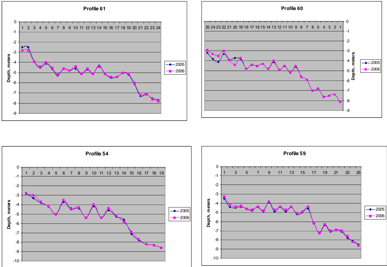
Fig.11. Samples of repeated profiles in the sand wave zone.
