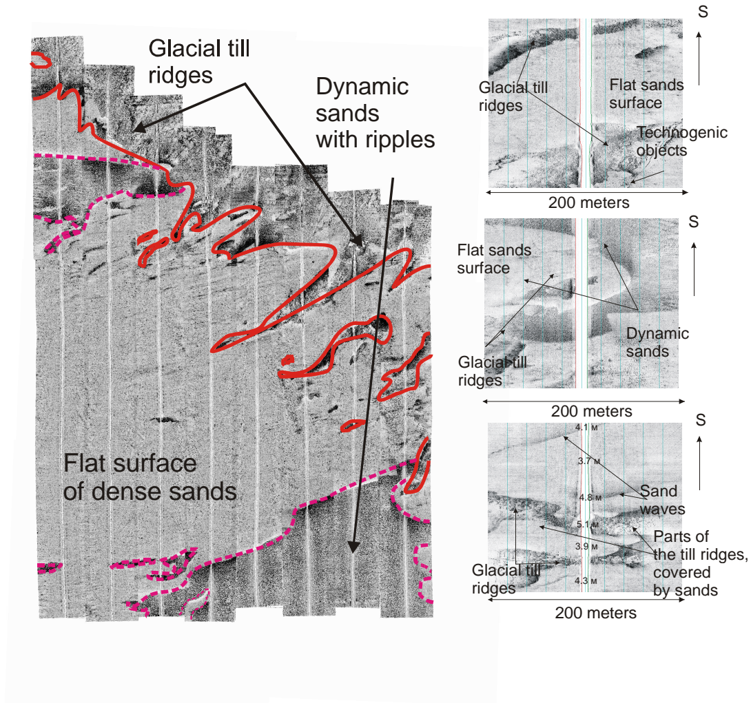
Fig.7.Side-scan mosaic and fragments of sonograms (in front of Solnechnoye village).
